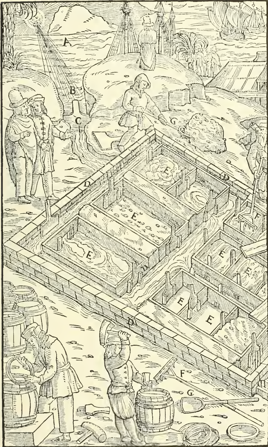
A—SEA. B—POOL. C—GATE. D—TRENCHES. E—SALT BASINS. F—RAKE. G—SHOVEL.
